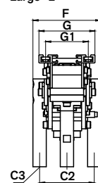
Track fastening Large "L"
