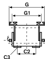
Track fastening Large "L"
