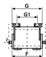
Track fastening Small "S"
